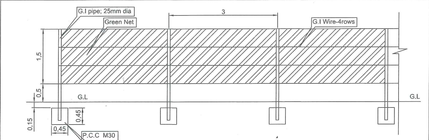
Details green net barricade
