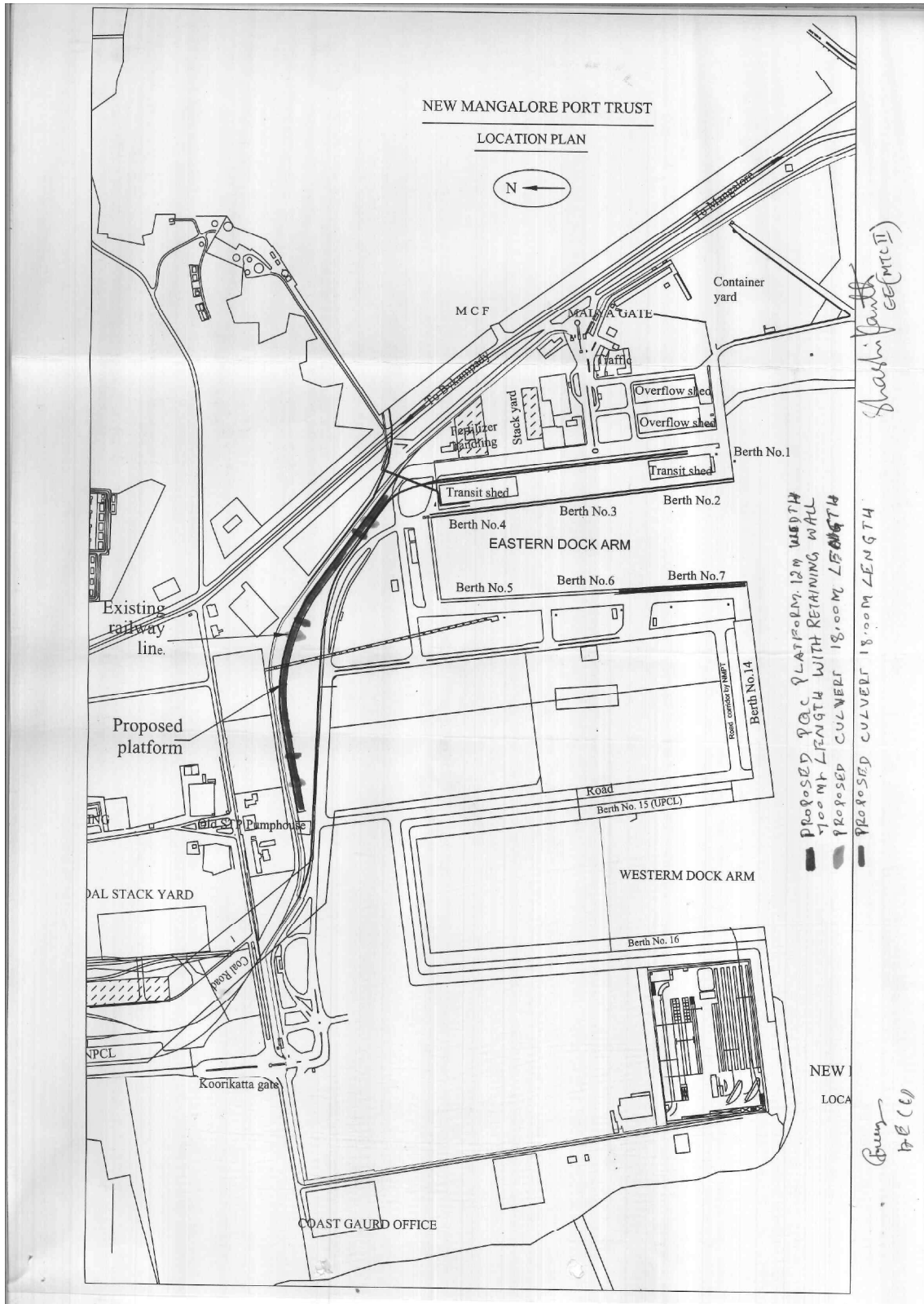
22/142-LP LOCATION PLAN
