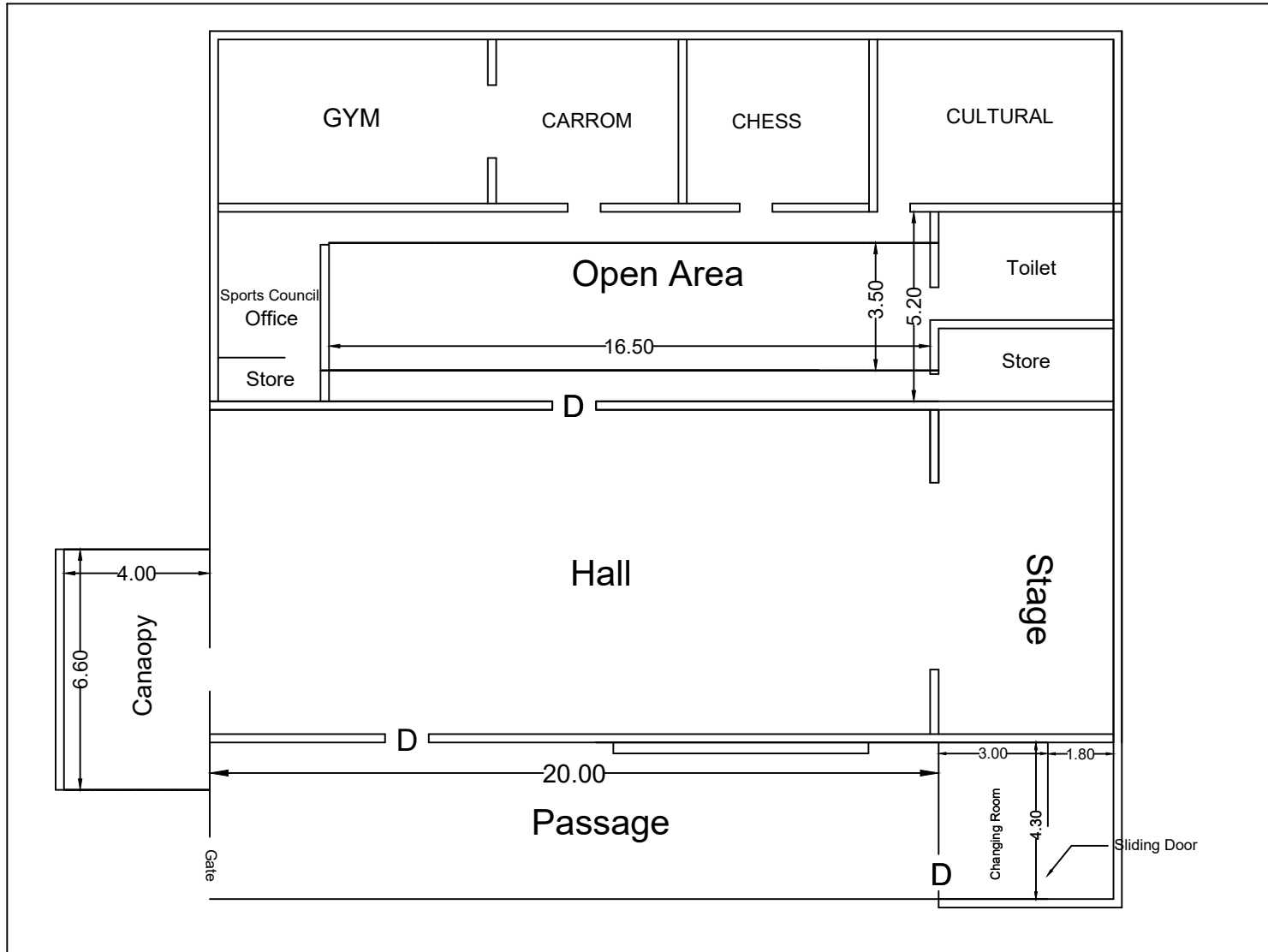
NEW MANGALORE PORT AUTHORITY Existing Plan of Sports Council Complex at NMPA Dwg. no. 5/323/BMR/002
