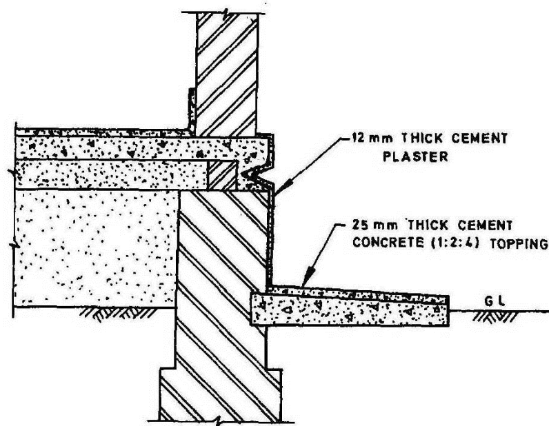
Fig 11 Anti-Termite construction (Stage 8)
