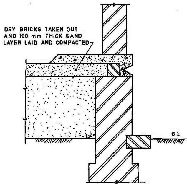
Fig 8 Anti-Termite construction (Stage 5)
