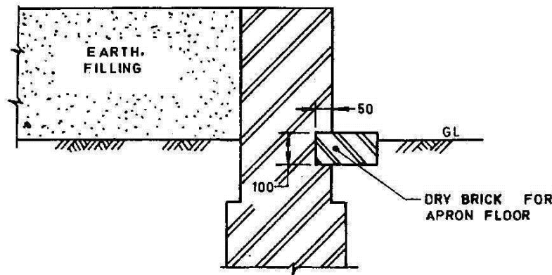
Fig 4 Anti-Termite construction (Stage 1)
