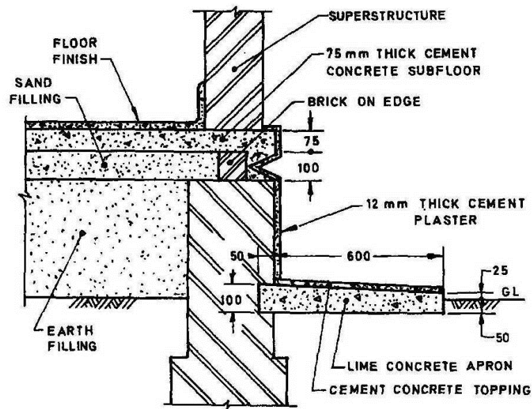
Fig 12 Anti-Termite construction – Final Recommendations
