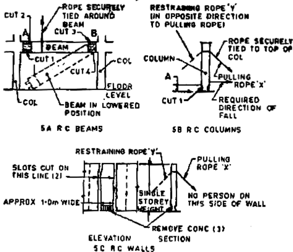
Fig 5 Hand demolition of in-situ concrete structure
