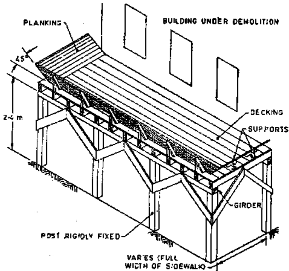
Fig 1 Typical sketch of sidewalk shed
