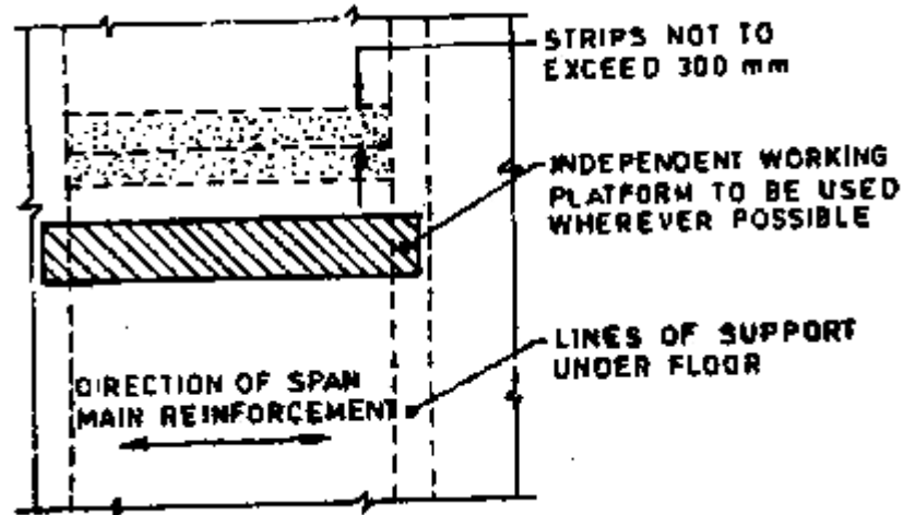
Fig 2 Demolition of reinforced concrete floors
