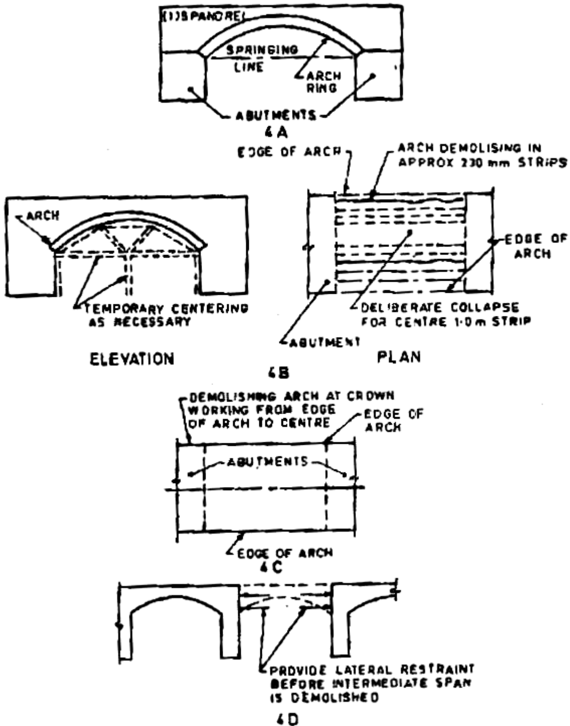
Fig 4 Demolition of masonry and brick arches
