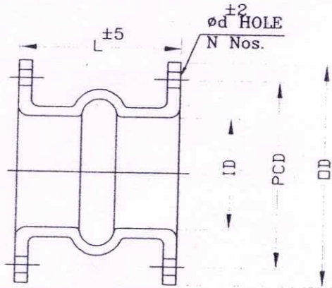
① RUBBER EXPANSION JOINT
